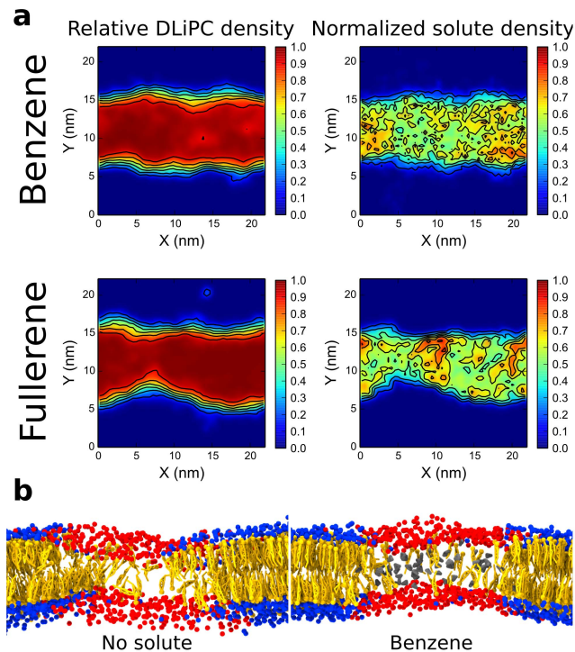
Figure 5. Mechanism of action of aromatic compounds. (a) Lipid and solute lateral distribution at 325 K, with high concentration of solute, expressed as relative DLiPC density normalized solute density. Aromatic solutes co-localize with unsaturated lipids. (b) Close-up view of the membrane centered on the L_d phase, in a system without solute (left) and in the presence of benzene (gray); cholesterol molecules are highlighted in orange. Benzene is found approximately at the same location as cholesterol. doi:10.1371/journal.pcbi.1003873.g005
