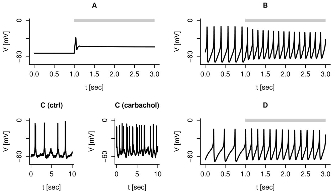
Figure 5. Paracrine effects on electrical activity. A: Simulation of application of 100 \mu M GABA to a silent cell (reproducing Fig. 7A in [12]). Default parameters except g_{KATP} = 0.021 nS/pF. GABA application was simulated by setting g_{GABAR} to 0.1 nS/pF during the period indicated by the gray bar. B: Simulation of application of 10 \mu M GABA to an active cell (reproducing Fig. 7B in [12]). GABA application was simulated by setting g_{GABAR} to 0.020 nS/pF during the period indicated by the gray bar. Other parameters took default values. C: Experimental recording of spiking electrical activity in the same human \beta -cell before (left) and during (right) application of carbachol (20 \mu M). D: Simulation of accelerated action potential firing due to carbachol application. Default parameters except g_{KATP} = 0.016 nS/pF. Carbachol application was simulated by increasing g_{leak} to 0.030 nS/pF during the period indicated by the gray bar. doi:10.1371/journal.pcbi.1003389.g005
