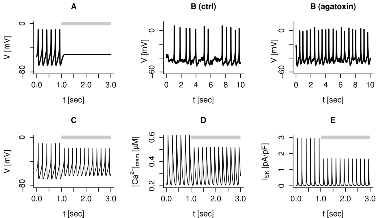
Figure 4. Block of L- and P/Q-type Ca^{2+} -channels affects electrical activity differently. A: Spiking electrical activity is suppressed by L-type Ca^{2+} -channel block in the model with default parameters, and g_{CaL} = 0 nS/pF during the period indicated by the gray bar. B: Spiking electrical activity is accelerated by the application of \omega -agatoxin IVA in human \beta -cells. Recordings from the same human \beta -cell in 6 mM extracellular glucose before (left) and during (right) application of 200 nM \omega -agatoxin IVA. C: Model simulation with default parameters of the membrane potential during spiking electrical activity under control conditions and after blockage of P/Q-type Ca^{2+} -channels ( g_{PQ} = 0 nS/pF during the period indicated by the gray bar). D: In the model, the peak submembrane Ca^{2+} -concentration [Ca^{2+}]_{mem} is lower when P/Q-type channels are blocked. E: The reduced [Ca^{2+}]_{mem} activate less SK-current when P/Q-type channels are blocked.
