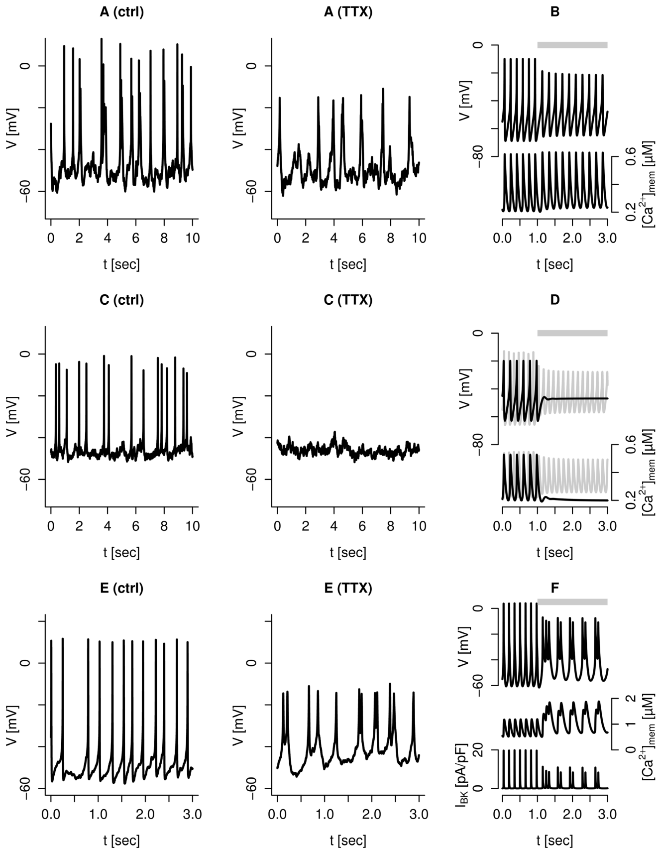
Figure 3. Tetrodotoxin (TTX, 0.1 \mu\text{g/ml} ) has different effects on electrical activity in human \beta -cells. A: TTX caused a reduction in action potential amplitude in this human \beta -cell. B: Simulation with default parameters showing V (upper trace, left axis) and [\text{Ca}^{2+}]_{\text{mem}} (lower trace, right axis), reproducing the data in panel A. C: TTX abolished action potential firing in this human \beta -cell. D: Simulations of V and [\text{Ca}^{2+}]_{\text{mem}} with default
