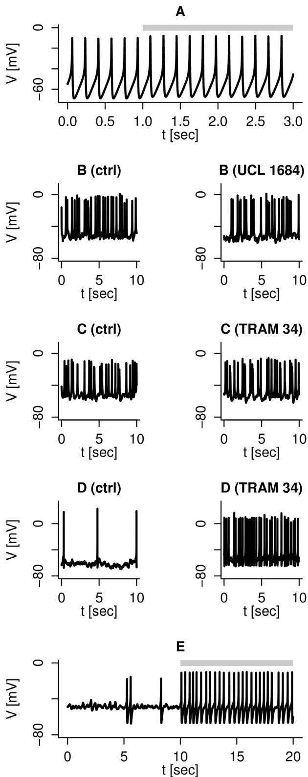
Figure 1. Heterogeneous responses to SK-channel block. Note the differences in time-scales. A: Simulation, with default parameters, showing no effect of SK-channels block ( g_{SK}=0 nS/pF during the period indicated by the gray bar). B: Experimental recording of spiking electrical activity in the same human \beta -cell before (left) and during (right) application of the SK1-3 channel antagonist UCL-1684 (0.2 \mu M). C: Experimental recording of spiking electrical activity in the same
