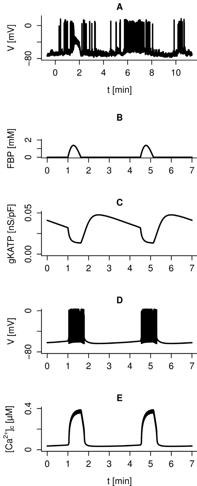
Figure 6. Metabolically driven slow waves of electrical activity and \text{Ca}^{2+} oscillations. A: Experimental recording of slow oscillations in action potential firing in a human \beta -cell exposed to 10 mM glucose. B–D: Simulation of slow bursting driven by glycolytic oscillations with glucose concentration G=10 mM and default parameters, except g_{Kv}=0.2 nS/pF, g_{SK}=0.02 nS/pF, g_{BK}=0.01 nS/pF. Oscillations in glycolysis create pulses of FBP (B), which via ATP production modulates K(ATP) channels in a periodic fashion (C). The rhythmic changes in
