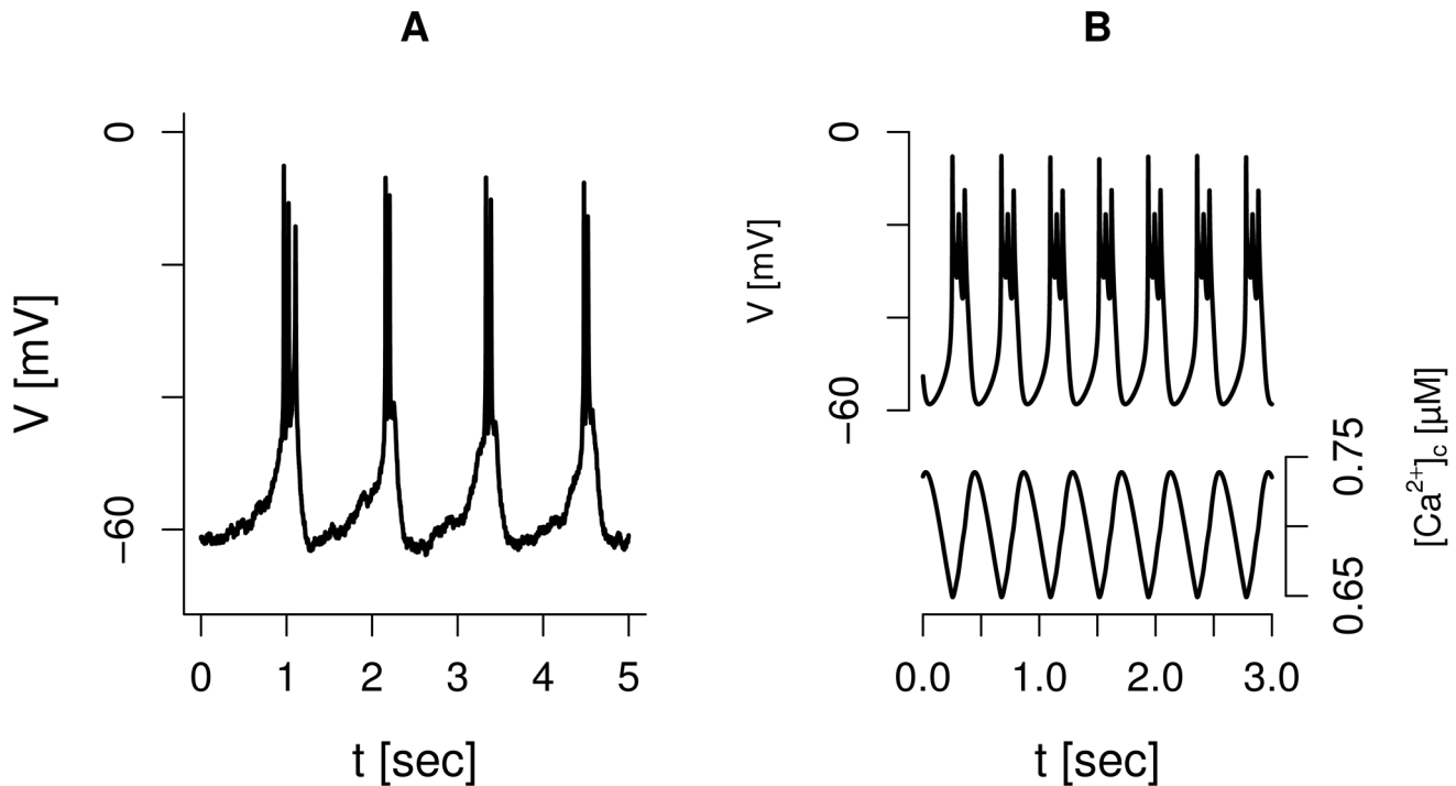
Figure 2. Bursting in human \beta -cell. A: Experimental recording of rapid bursting in a human \beta -cell. B: Simulation of bursting driven by [Ca^{2+}]_c via SK-channels. Default parameters except g_{SK} = 0.03 nS/pF, g_{Kv} = 0.25 nS/pF, n_{XPQ} = -10 mV. doi:10.1371/journal.pcbi.1003389.g002
