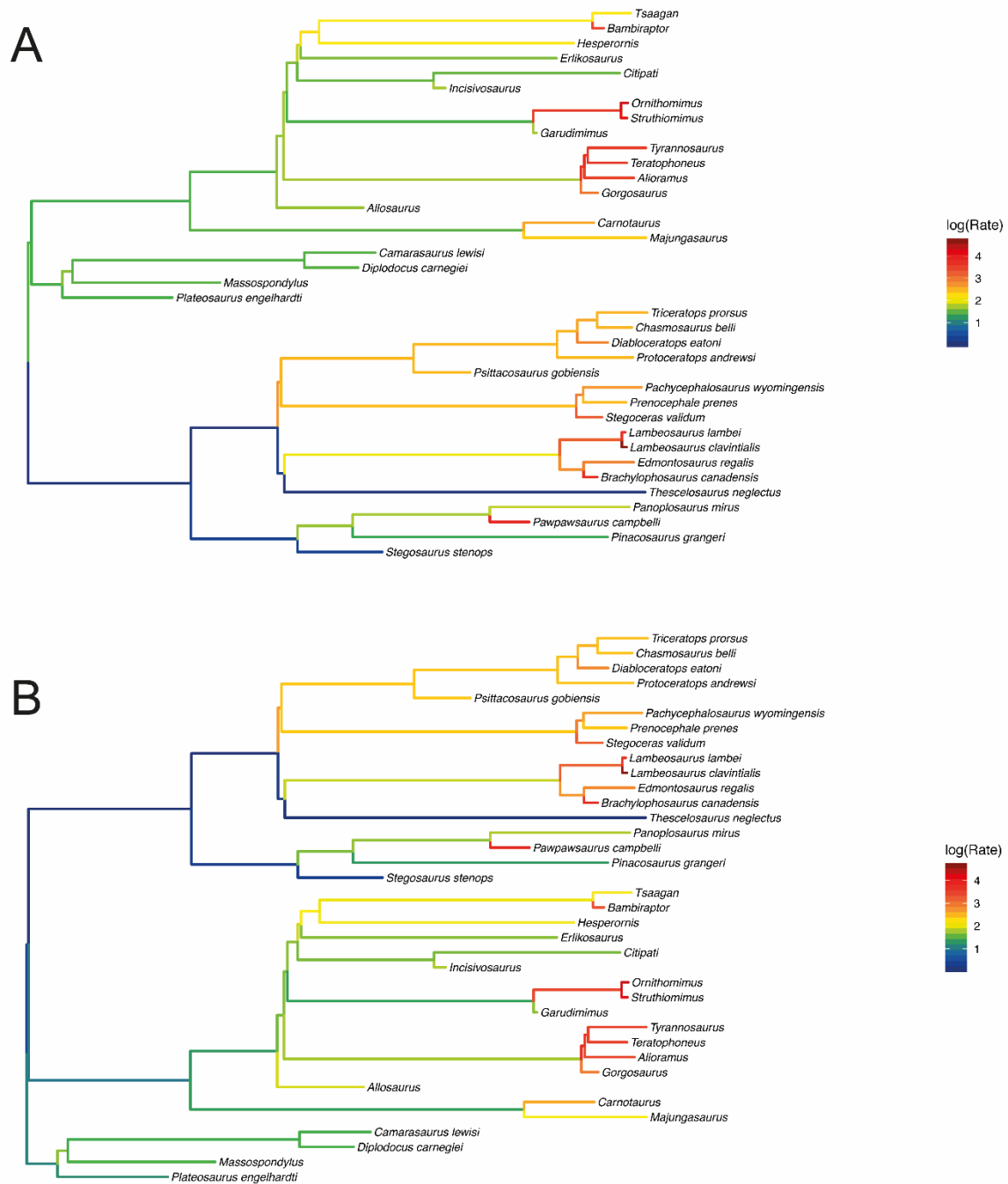
S25 Fig. Estimation of rates of squamosal bone evolution. Modelled using the (A) traditional phylogenetic hypothesis and (B) Ornithoscelida hypothesis under a variable-rates Brownian motion model of evolution. Data and code archived at www.github.com/rnfelice/Dinosaur_Skulls .
