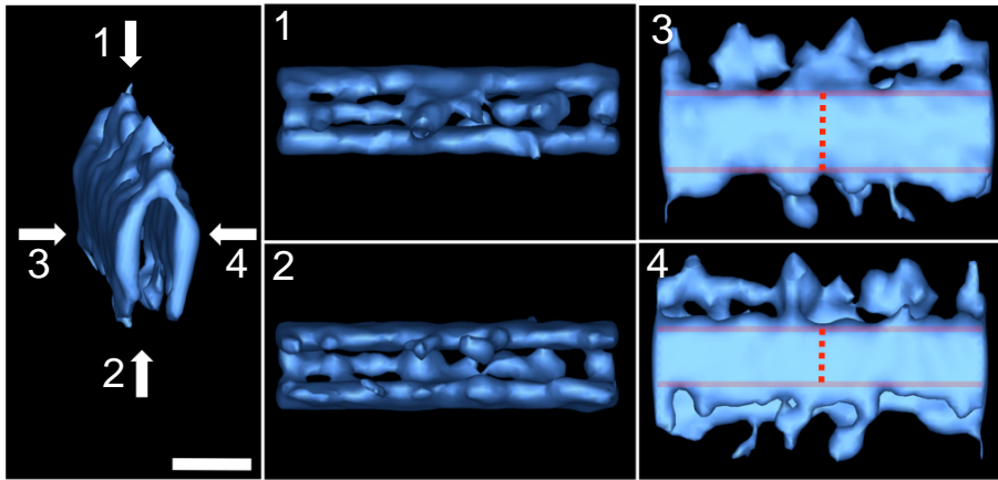
Figure S8. Sub-tomogram averaging of bacterial microtubules.
