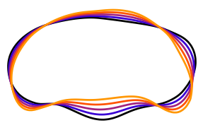
Shape Mode 3 (2.9% of total variance)
