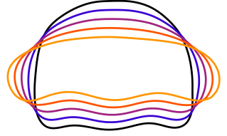
Shape Mode 2 (19.6% of total variance)
