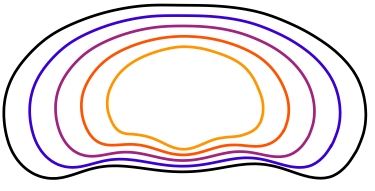
Shape Mode 1 (73.9% of total variance)
