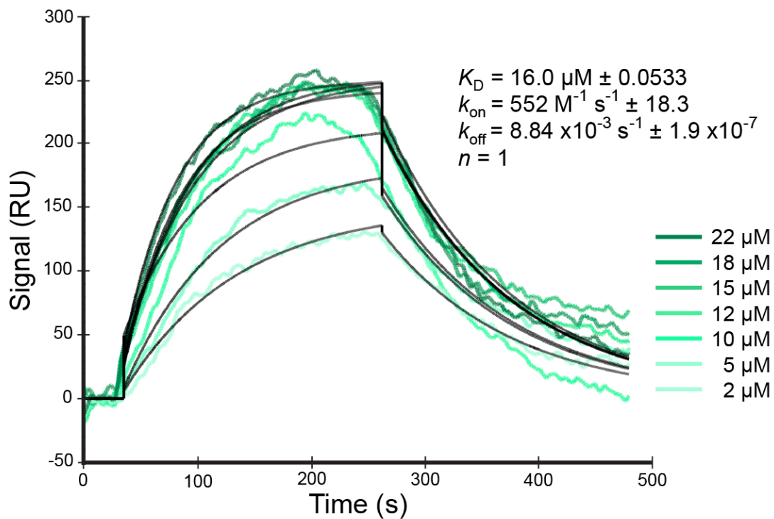
S19 Fig. Surface plasmon resonance (SPR) experiments testing the minimal adhesive unit for mouse PCDH24 and CDHR5. Raw data from the SPR experiment performed on mm PCDH24 EC1-2Fc and mm CDHR5 EC1-2 shown in green gradient from lowest concentration (light green) to highest concentration (dark green) of mm CDHR5 EC1-2, with fits in black. The average affinity K_D and rates ( k_{\text{on}} and k_{\text{off}} ) are indicated ( n = 1 ). Values were obtained from a kinetic analysis of the raw data (S13 Data).
