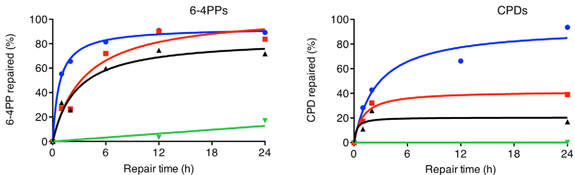
Figure 4. CUL4A-dependent excision of UV lesions from internucleosomal DNA. The excision of 6-4PPs (left) and CPDs (right) was determined in whole chromatin (A) and MNase-insoluble (4 U/ \mu l) core particles (B) of HeLa cells transfected with the indicated siRNA reagents and exposed to UV light (10 J/m 2 ). Relative amounts of each photolesion were determined at the indicated times by enzyme immunoassay (mean values of 3–5 independent determinations). Subsequently, the excision of UV lesions from MNase-solubilizable internucleosomal DNA (C) was calculated by subtracting the photolesions in the insoluble core particle fraction from those found in the whole chromatin. The initially delayed 6-4PP excision in a DDB2-depleted background (siDDB2) fits with the reported repair kinetics of XP-E cells [21,22]. doi:10.1371/journal.pbio.1001183.g004
