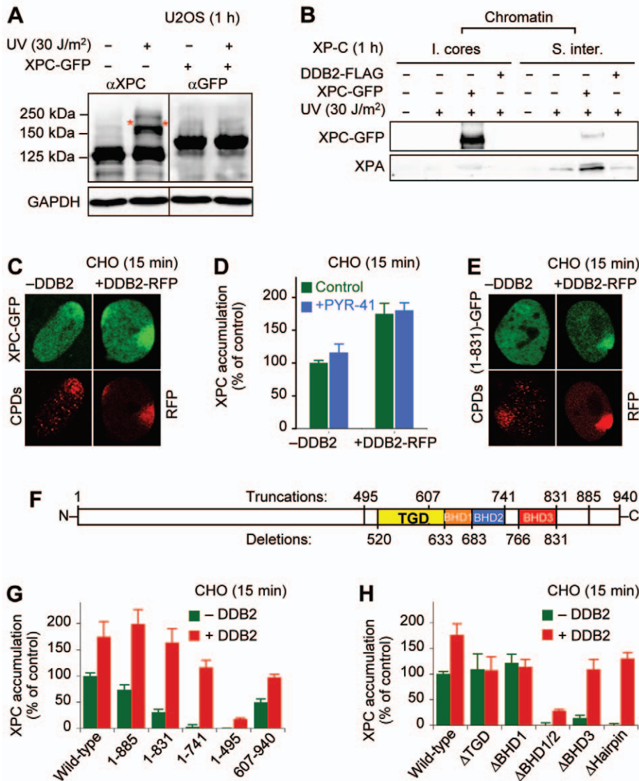
Figure 5. Ubiquitin-independent XPC recruitment by UV-DDB. (A) Minimal ubiquitylation of XPC-GFP, compared to endogenous XPC, demonstrated by Western blotting. (B) UV-dependent binding of XPC-GFP primarily to MNase-insoluble (4 U/ \mu l) core particles ("l. cores") of XP-C fibroblasts. The subsequent XPC-dependent recruitment of XPA occurs mainly to solubilizable internucleosomal DNA ("S. inter."). (C) XPC-GFP relocation to UV-irradiated areas of DDB2-deficient CHO cells. UV lesion spots were visualized with CPD antibodies or by monitoring DDB2-RFP intensity. (D) XPC-GFP relocation to UV lesions stimulated by co-expression of DDB2-RFP. GFP signals at UV lesion spots ( N=30 ) were quantified, normalized against the nuclear background, and expressed as a percentage of controls (XPC alone). (E) DDB2-stimulated relocation of XPC 1-831 -GFP to UV-irradiated areas. (F) Domain structure of human XPC (see Figure S4B for truncations and deletions). (G) Recruitment of XPC-GFP truncates. Fluorescence spots co-localizing with UV lesions ( N=30 ) were normalized and expressed as a percentage of control values (full-length XPC alone). (H) Recruitment of XPC-GFP deletions to UV lesions ( N=30 ). doi:10.1371/journal.pbio.1001183.g005
