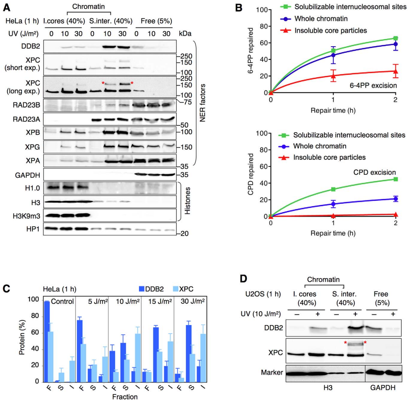
Figure 1. Preferential binding of UV-DDB to internucleosomal DNA. (A) The distribution of NER factors was analyzed in the chromatin of HeLa cells by MNase digestion (4 U/ \mu l) and immunoblotting. GAPDH, glyceraldehyde-3-phosphate dehydrogenase; H3K9m3, trimethylated histone H3; HP1, heterochromatin protein 1. The asterisks in the long exposure denote ubiquitylated XPC. "I. cores," insoluble core particles. "S. inter.," solubilized internucleosomal sites. "Free," proteins not bound to chromatin. The numbers in parentheses indicate the percentages of each fraction loaded onto the gel. (B) Initial excision of UV lesions from distinct nucleosomal sites measured by MNase treatment (4 U/ \mu l) and enzyme immunoassay (average of three independent experiments). The repair of 6-4PPs and CPDs in digested internucleosomal DNA (squares) was calculated by subtracting the photolesions in core particles (triangles) from those found in whole genomic DNA (circles). The UV dose was 10 J/m 2 . (C) Quantification of the UV-dependent translocation of UV-DDB and XPC from the pool of free (F) proteins to solubilizable internucleosomal sites (S) and insoluble core particles (I). Relative amounts of DDB2 and XPC (mean values of 3–5 experiments) were calculated (see Text S1) from Western blot quantifications and corrections for differences in the loading volume as indicated in panel A. (D) UV-dependent relocation of DDB2 and XPC in p53-proficient U2OS cells determined by MNase digestion (4 U/ \mu l). doi:10.1371/journal.pbio.1001183.g001
