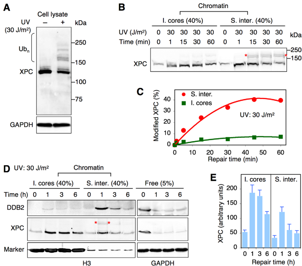
Figure 2. Differential XPC ubiquitylation in chromatin. (A) UV-dependent ubiquitylation of XPC protein visualized by an immunoblot of HeLa whole-cell lysates 15 min after UV irradiation (30 J/m 2 ). Ub n , ubiquitylated forms of XPC. (B) The chromatin of HeLa cells was dissected by MNase digestion (4 U/μl) at different times after UV exposure to compare the ubiquitylation of XPC bound to the core particle fraction ("I. cores") or internucleosomal DNA ("S. inter."). (C) Quantitative comparison of ubiquitylated XPC relative to total XPC associated with either solubilizable (4 U/μl) internucleosomal sites ("S. inter.") or MNase-resistant core particles ("I. cores") at the indicated times after UV irradiation (mean values of two independent determinations). (D) Representative blot illustrating the DDB2 degradation and long-term binding of XPC to the insoluble core particle fraction ("I. cores") after UV exposure. (E) Quantification of the time-dependent XPC distribution in the chromatin of UV-exposed HeLa cells. XPC amounts in the core particle fraction ("I. cores") and at internucleosomal sites ("S. inter.") were calculated from Western blots followed by corrections for the different loading as indicated in panel D (mean values of three independent determinations). doi:10.1371/journal.pbio.1001183.g002
