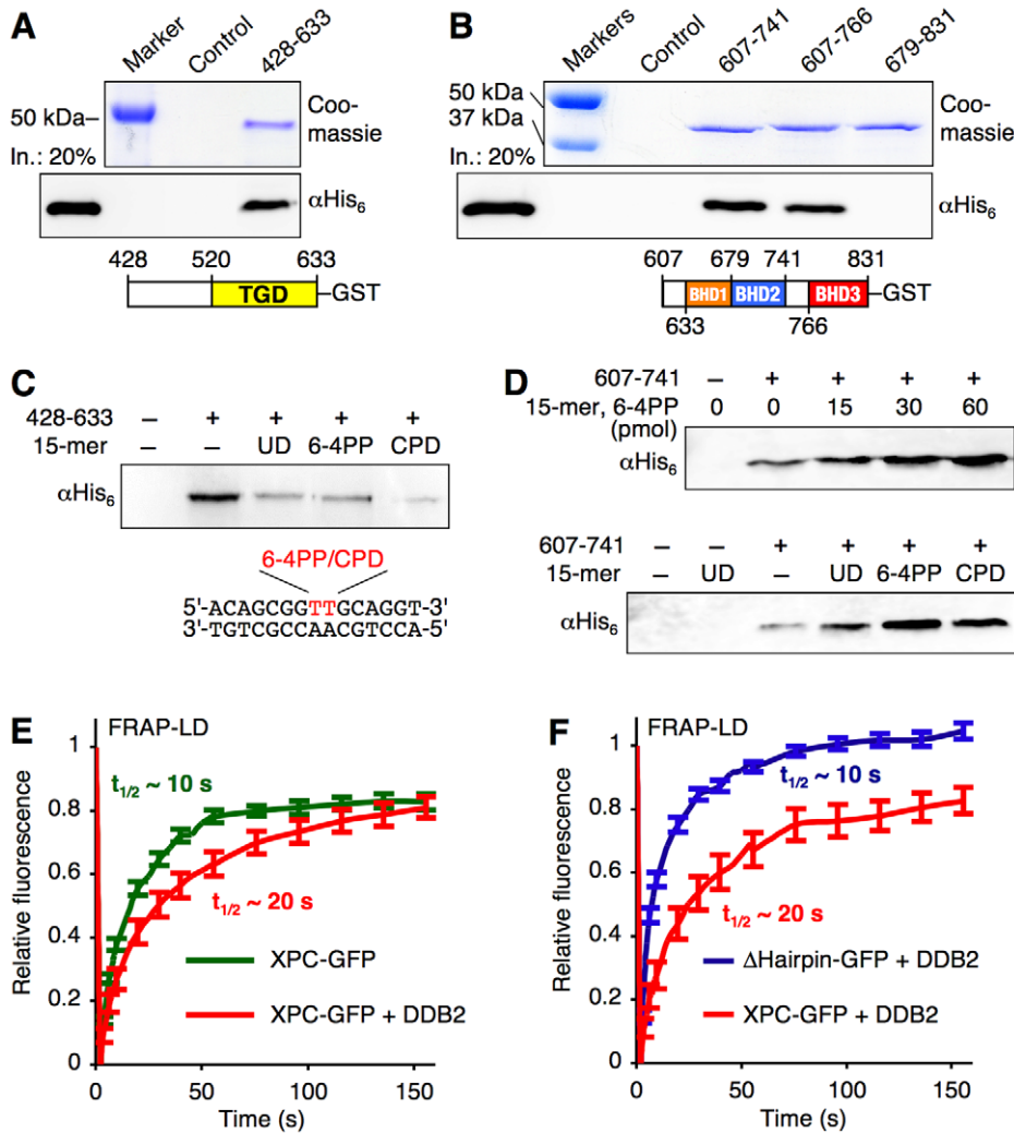
Figure 6. Dynamic DDB2-XPC interactions in chromatin. (A) DDB2 association with the TGD motif of XPC. Purified UV-DDB-His 6 (120 pmol) was incubated with XPC 428–633 -GST (120 pmol) and probed by adding glutathione beads. XPC 428–633 -GST in the pull-down fraction was visualized by Coomassie staining whereas antibodies against His 6 detected interacting DDB2. An input (“In.”) control displays 20% of total DDB2 in each incubation. (B) DDB2 association with XPC 607–741 -GST and XPC 607–766 -GST, both containing the BHD1/BHD2 motifs. (C) Interaction between DDB2 and XPC 428–633 -GST inhibited by a 15-mer DNA duplex (120 pmol). UD, undamaged. The 15-mer sequence is shown with the 6-4PP or CPD position in red. (D) Interactions between DDB2 and XPC 607–741 -GST are stimulated by a 15-mer DNA duplex (top panel: 15–60 pmol; bottom panel: 120 pmol). (E) Dissociation of XPC-GFP from UV lesions in CHO cells measured by FRAP-LD ( N=15 ; \pm s.e.m.). Half-lives were estimated from the fluorescence recovery curves. (F) DDB2 is unable to stabilize the \Delta Hairpin deletion at UV lesions in FRAP-LD assays ( N=15 ). A control fluorescence recovery in the absence of DDB2 is not possible because the \Delta Hairpin deletion alone fails to relocate to DNA damage. doi:10.1371/journal.pbio.1001183.g006
