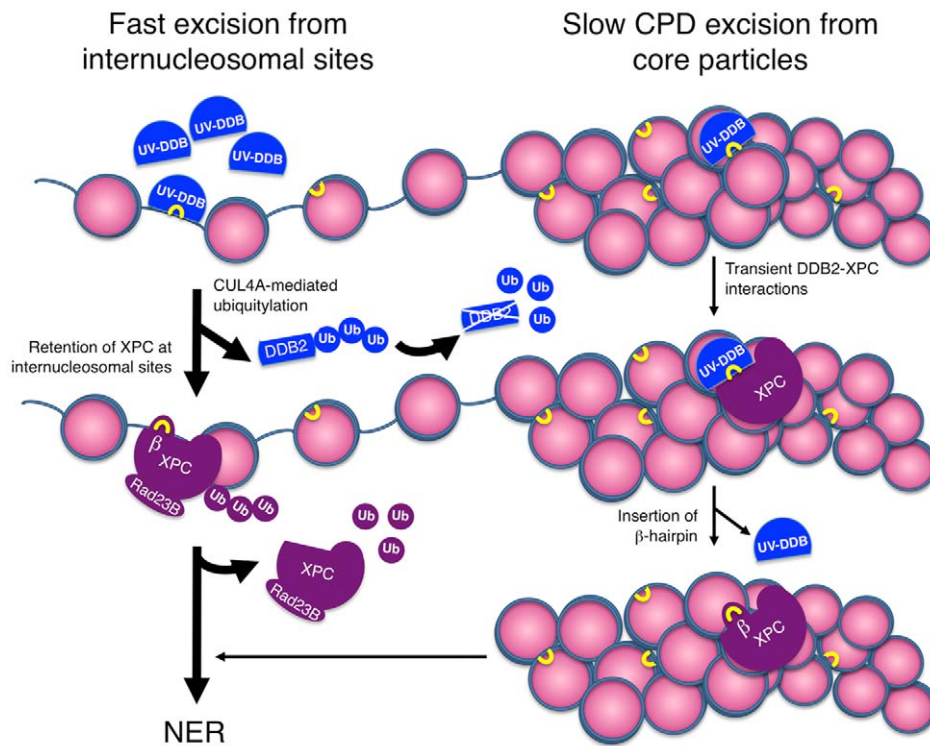
Figure 7. Novel regulatory principle in DNA repair. Left , ubiquitin-dependent prioritization of DNA repair to internucleosomal sites. The preferential UV-DDB accumulation on internucleosomal DNA leads to ubiquitylation of the XPC partner by CUL4A ligase. This modification promotes the XPC retention at internucleosomal sites, thus reducing its association with nucleosome core particles. The implementation of this ubiquitin code is required for the fast initial excision of UV lesions from internucleosomal DNA. Concomitantly ubiquitylated DDB2 is degraded, but XPC protein is protected from proteasome activity by RAD23B [47]. Right , ubiquitin-independent priming platform. UV-DDB undergoes very transient interactions with the TGD and BHD1 motifs of XPC, thereby facilitating the insertion of a \beta -hairpin subdomain, to hand over the substrate to the downstream NER process. This ubiquitin-independent substrate handover is required, regardless of nucleosome localization, for the excision of CPDs that on their own induce minimal distortions of the DNA duplex and, hence, are not recognizable by XPC alone. Ub, ubiquitin; \beta , \beta -hairpin of XPC. UV lesions are indicated with yellow brackets.
