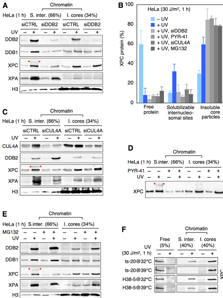
Figure 3. Ubiquitin-dependent XPC retention on internucleosomal DNA. (A) Comparison between internucleosomal sites (“S. inter.”) and core particles (“I. cores”) illustrating that a DDB2 depletion alters the chromatin distribution of DDB1, XPC, and XPA. DDB2 was down regulated by transfection with siRNA and the chromatin was dissected by MNase digestion (4 U/ \mu l) 1 h after UV irradiation (30 J/m 2 ); siCTRL, control RNA. (B) Quantitative assessments demonstrating the abnormal XPC distribution (reduced retention at solubilizable internucleosomal sites and increased binding to insoluble core particles) after inhibition of the ubiquitylation pathway by different treatments. The XPC translocation to the indicated nucleosome fractions (mean values of 3–5 experiments) was determined from Western blots with corrections for the differences in loading as indicated in panel A (see Text S1). (C) Representative blot illustrating the altered XPC and XPA distribution following CUL4A depletion (UV: 30 J/m 2 ). (D) Representative blot showing that a treatment with the E1 inhibitor PYR-41 reduces the XPC retention at internucleosomal sites without diminishing its UV-dependent accumulation in the core particle fraction. The UV dose was 30 J/m 2 . (E) Representative blot illustrating that MG132 reduces the UV-dependent XPC retention and the subsequent recruitment of XPA to internucleosomal sites (UV: 30 J/m 2 ). (F) E1 inactivation in ts-20 cells (at 39°C) suppresses the UV-dependent XPC retention at internucleosomal sites (“S. inter.”). This response is not observed at 32°C or in corrected H38-5 cells. The available antibodies are unable to detect ubiquitylated mouse XPC. doi:10.1371/journal.pbio.1001183.g003
