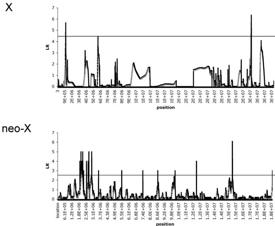
Figure 2. The Maximized Composite Likelihood Surface Calculated for Genes from the Ancestral X and the Neo-X Chromosome
