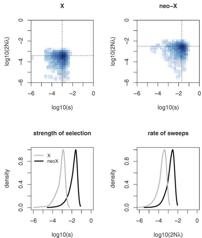
Figure 3. Approximate Bayesian Estimation of the Rate of Adaptive Substitutions ( 2N_e\lambda ) and Their Average Effect on Fitness ( s ) for Genes from the Ancestral X and the Neo-X Chromosome
