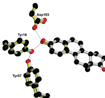
Superimposition of complexes formed between the active site of ketosteroid isomerase and two transition-state analogs.
