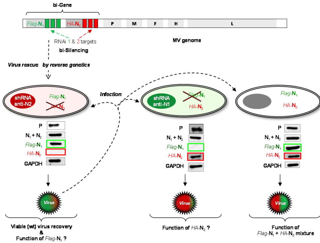
S8 Fig. Principle of biG-biS MeV viruses selective expression of the duplicated N1 and N2 gene according to the Vero cell host (see [3] for details).
