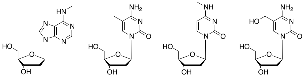
N 6 -Methyl dA
