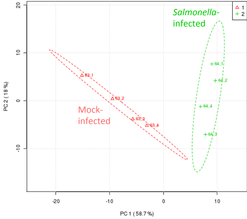
Score Plot
