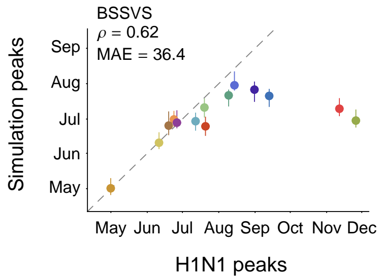
Figure S9: Correlation among observed H1N1 peaks and simulated peaks based on the BSSVS estimates. The Spearman rank correlation ( \rho ) and mean absolute error (MAE; in days) for all locations except for Mexico is shown at the top left. The data points are colored according to the air communities represented in Fig. 1 in the main text.
