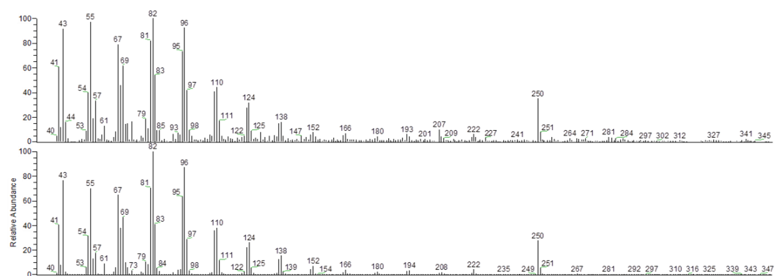
S4 Fig. Mass spectrum of Z9-18:Ac from an extract of terminalia of a P. archon male in comparison to that of the synthetic material.
