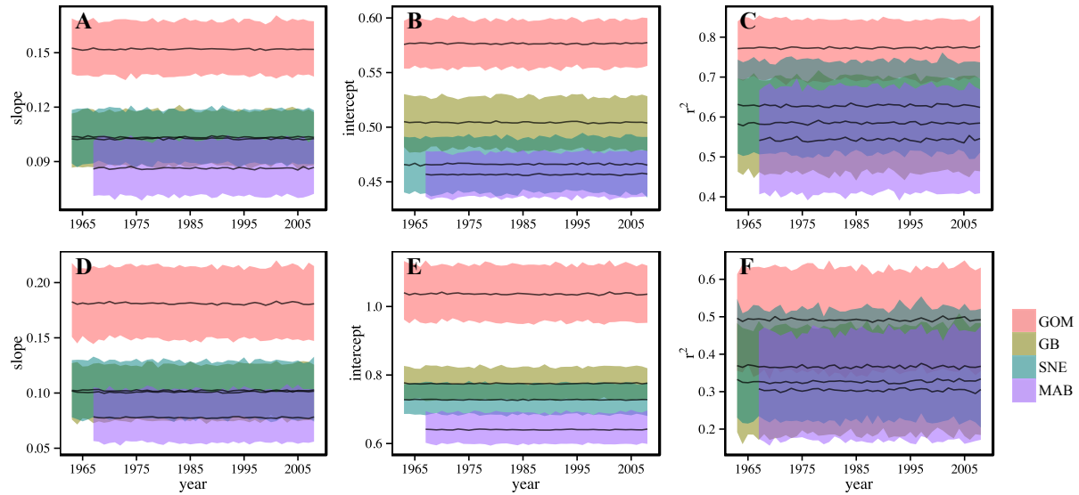
Figure S2. Mean AOR regression statistics for simulations with negative binomial (NB) parameters held constant. Results are given for relationships estimated with global mean abundance, GMA (A-C) and local mean abundance, LMA (D-F). In each plot, 95% confidence intervals are color-coded by region. Regions included are the Gulf of Maine (GOM), Georges Bank (GB), Southern New England (SNE), and the Mid-Atlantic Bight (MAB).
