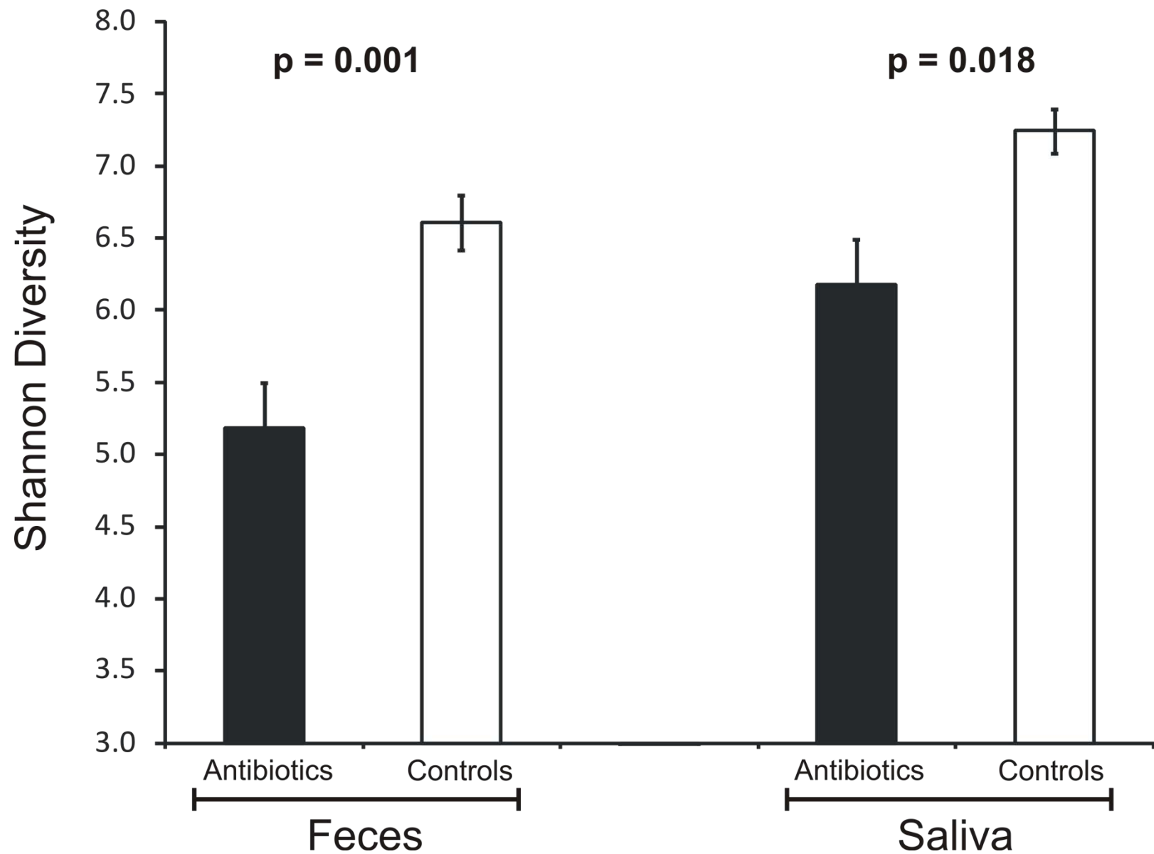
S5 Fig: Shannon diversity index values ( \pm standard error) for fecal and salivary bacterial biota based on 16S rRNA. P-values are represented above each diagram, and values \leq 0.05 are represented in bold.
