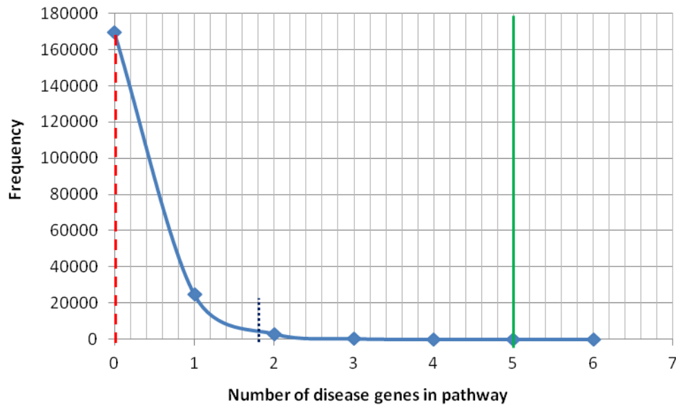
Figure S1: Association of nasopharyngeal carcinoma to KEGG pathway hsa04514 (cell adhesion molecules). Curve depicts the amount of randomly selected genes found in each pathway through 1,000 random runs. X-axis represents the number of genes in the pathway, while the Y-axis represents the frequency. The solid line depicts the actual number of NPC genes in pathway hsa04514 (5), while the dashed line depicts the median of all random runs (0). p-value is 0.01E-4. Any value higher than the dotted line is significant ( < 0.05 ).
