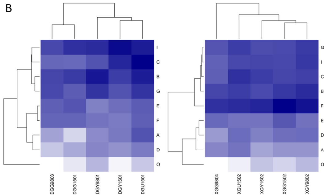
Figure S6. ABC transporter gene family distribution and expression cluster.
