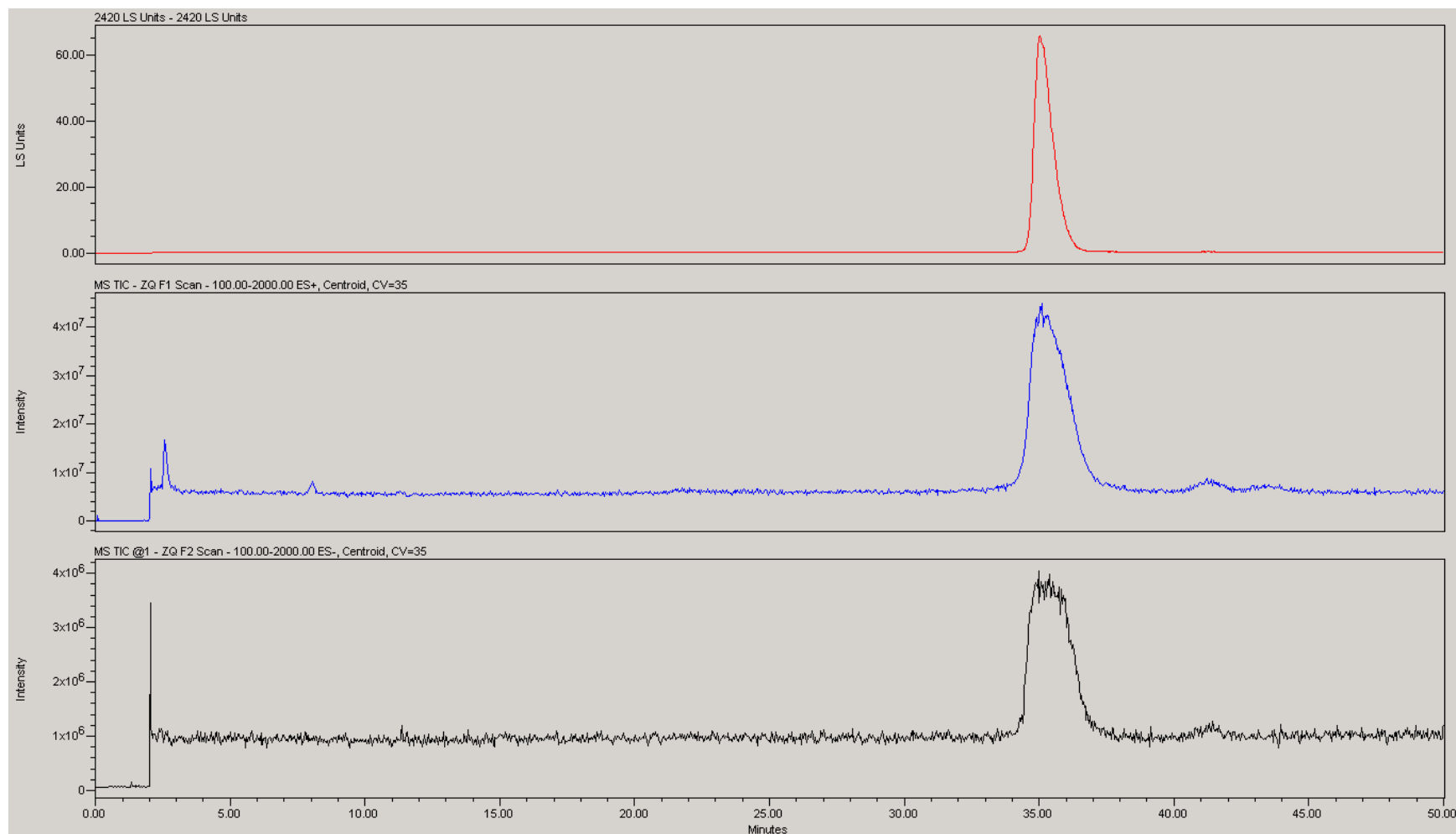
Figure S16. MS and analytical chromatograms of GA-XIII ( 3 ) as detected by ELSD, MS ES+ TIC and MS ES- TIC mode, respectively.
