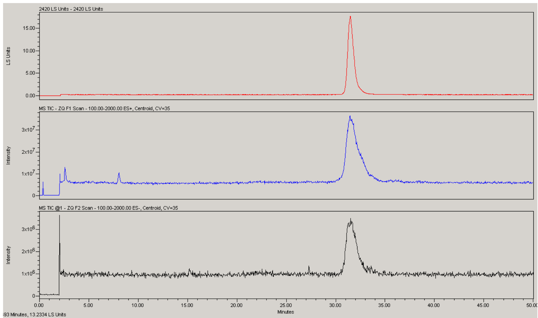
Figure S11. MS and analytical chromatograms of GA-XIV ( 4 ) as detected by ELSD, MS ES+ TIC and MS ES- TIC mode, respectively.
