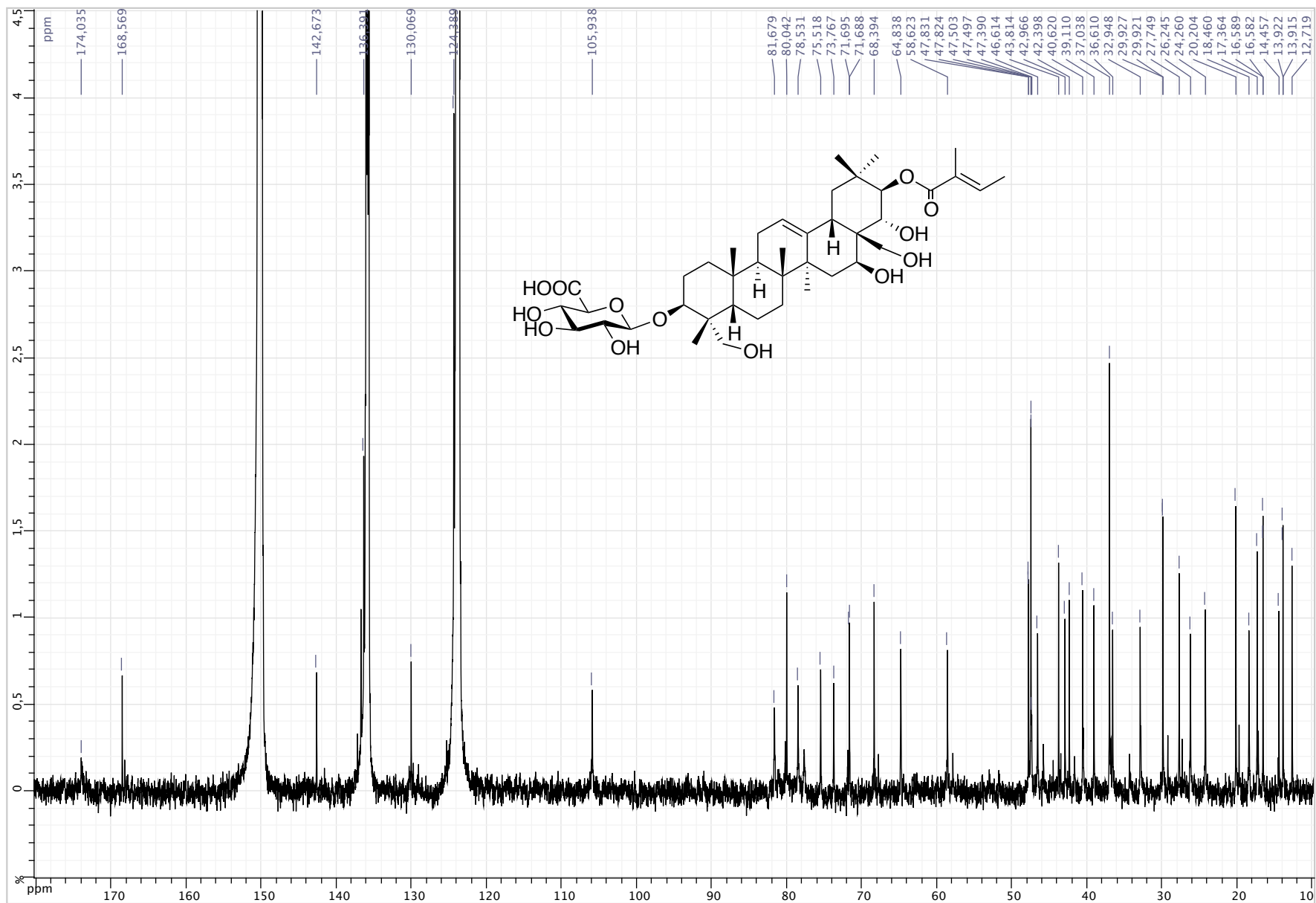
Figure S5. ^{13}\text{C} NMR spectra of GA-IV (2) in \text{C}_5\text{D}_5\text{N} (150 MHz).
