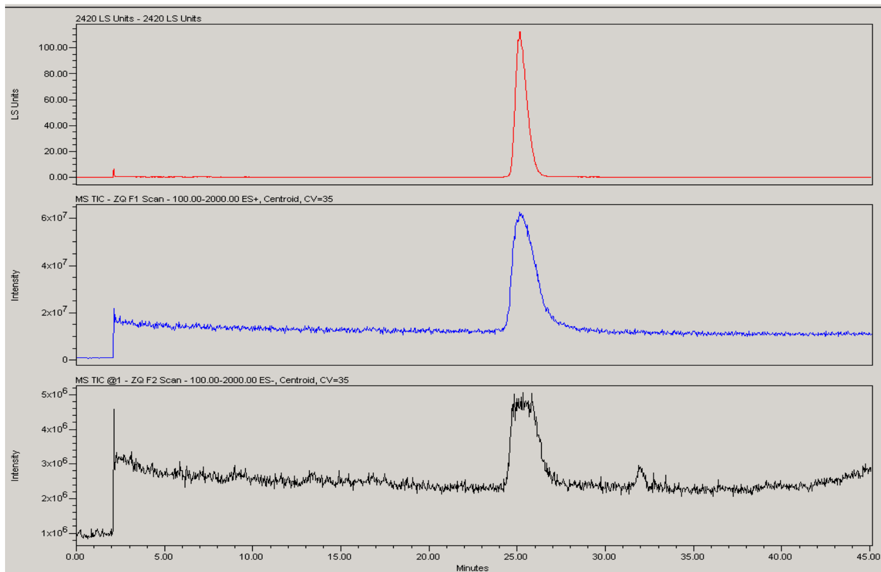
Figure S1. MS and analytical chromatograms of GA-IV ( 2 ) as detected by ELSD, MS ES+ TIC and MS ES- TIC mode, respectively.
