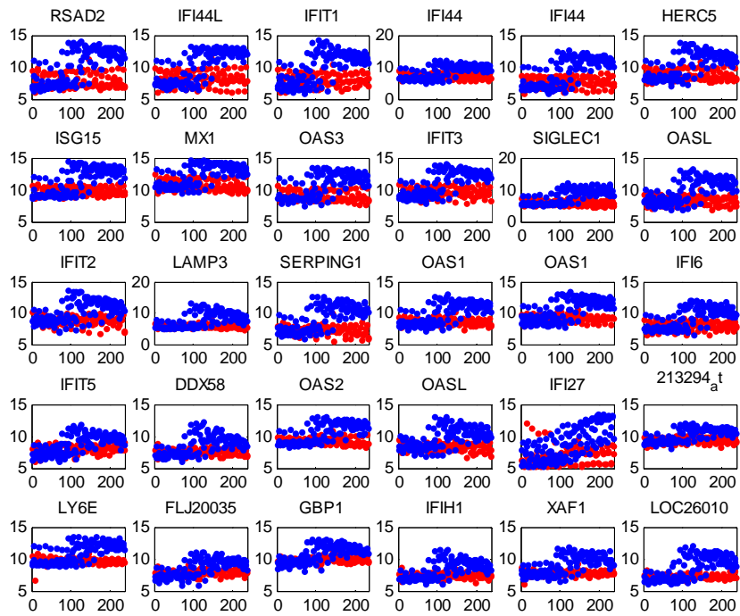
Figure s2. Variation over time of the expression of the top 30 individual genes which make up the Influenza factor.
