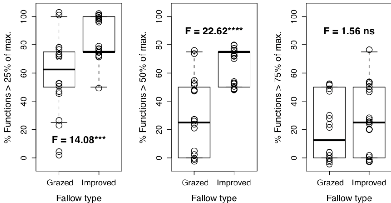
Figure S1 Variation among fallow types in ecosystem multi-functionality in terms of the proportion of ecosystem functions above 25, 50, and 75% of respective function maxima; points are jittered slightly for greater clarity. Statistics presented from one-way ANOVA with d.f. = 1, 37. * = P < 0.05 , ** = P < 0.01 , *** = P < 0.001 , **** = P < 0.0001 , ns = P > 0.1 .
