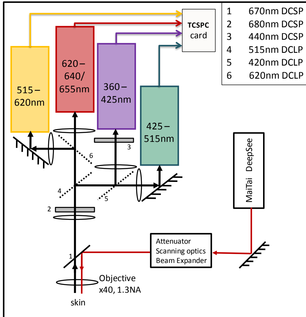
Figure S4- Schematic of instrument. Key-DCSP - dichroic short pass, DCLP – dichroic long pass
