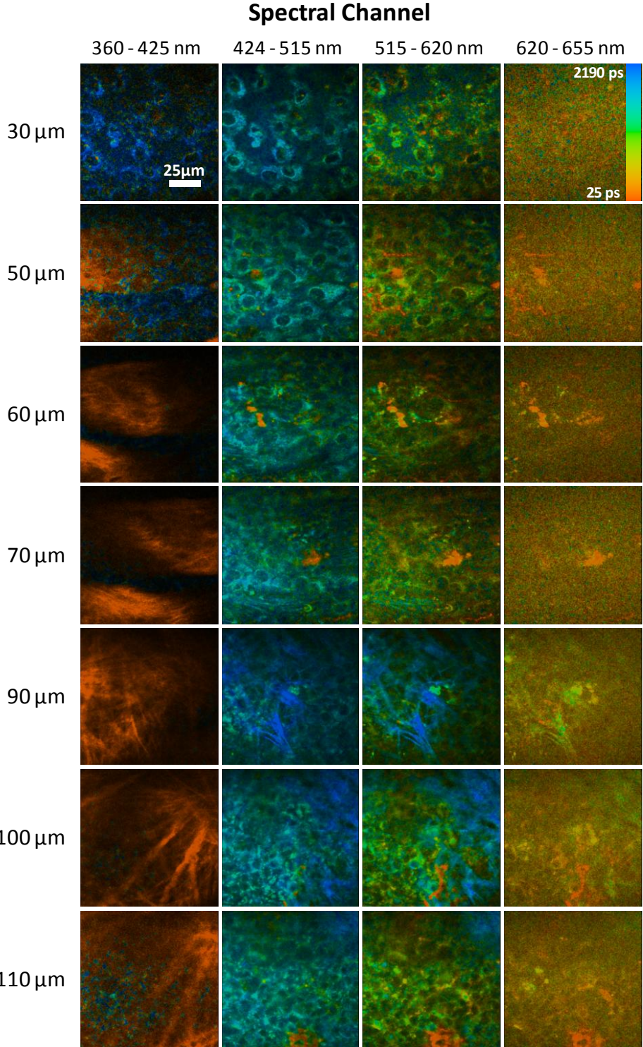
Figure S2 - Multispectral FLIM images taken at multiple depths from (a) a nodular/superficial BCC and (b) a nodular/pigmented BCC.
