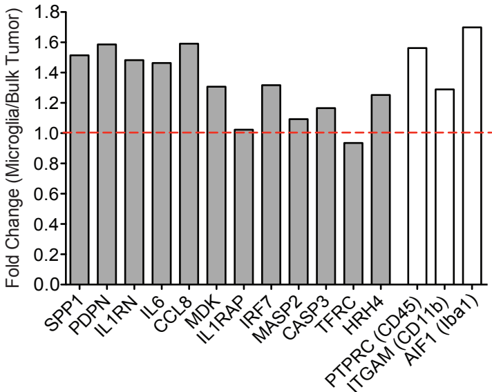
Figure S5. Expression of survival-associated immune response-related genes in glioma infiltrating microglia/macrophages (GIM) relative to bulk tumor. Grey bars indicate immune genes identified by CoxBoost analysis (Table 1). White bars indicate common microglia/macrophage markers. The red dotted line denotes a 1-fold change, hence no difference in gene expression between GIM and bulk tumor.
