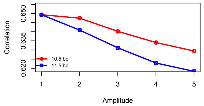
Oct4-Zfx
