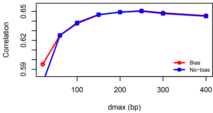
Oct4-Zfx
