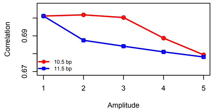
STAT3-Klf4
