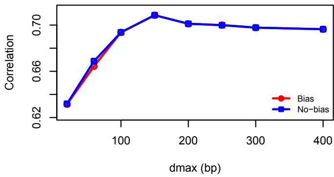
STAT3-Klf4
