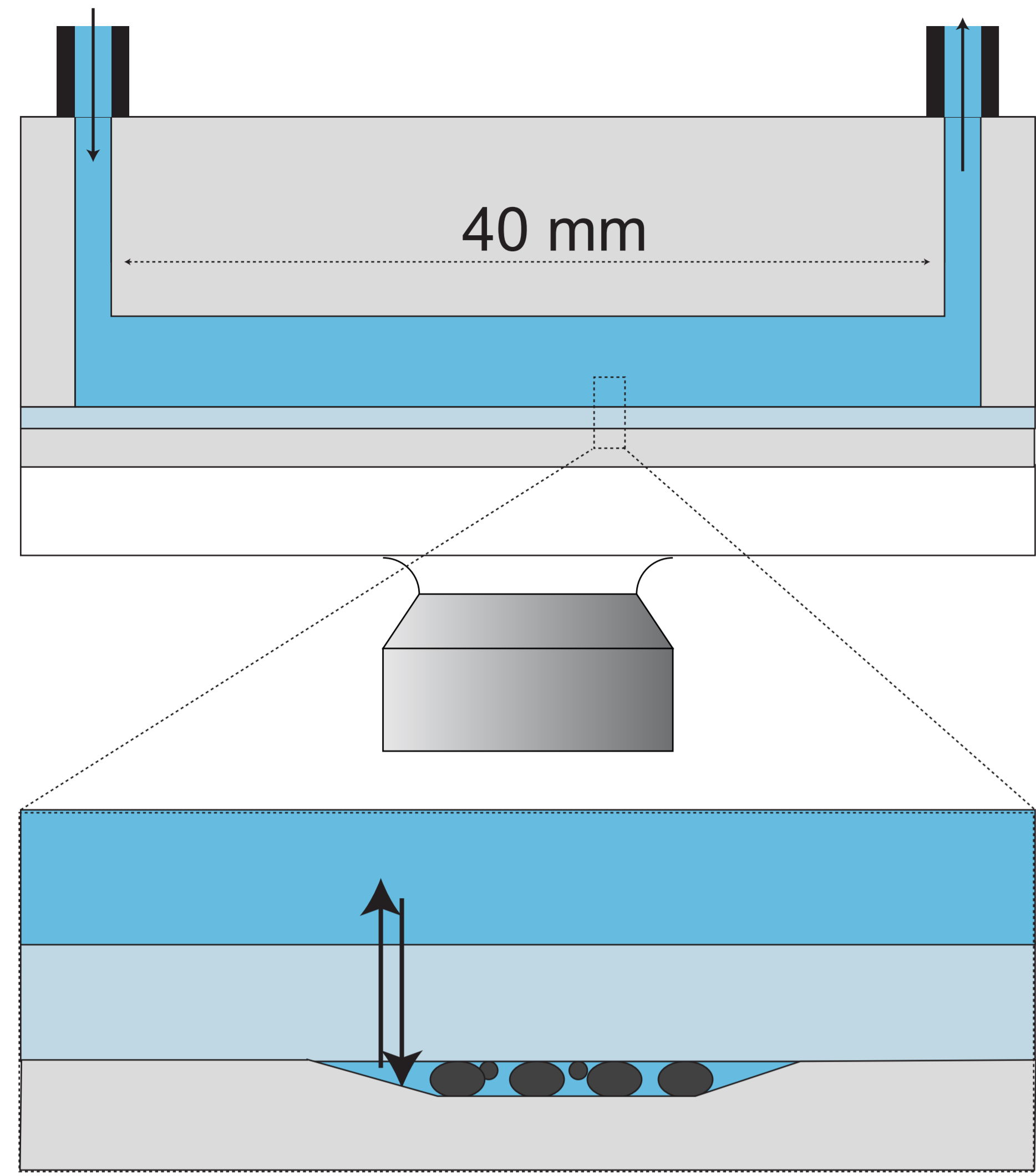
Flow chamber
