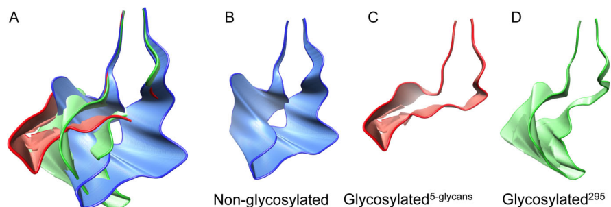
Figure 4. Representation of the range of movement of the V3 loops for the first principal component. The range of movement is presented for (A) all systems, (B) non-glycosylated, (C) glycosylated 5-glycans , and (D) glycosylated 295 trajectories. The shaded colors represent the intermediate positions between the extremes.
