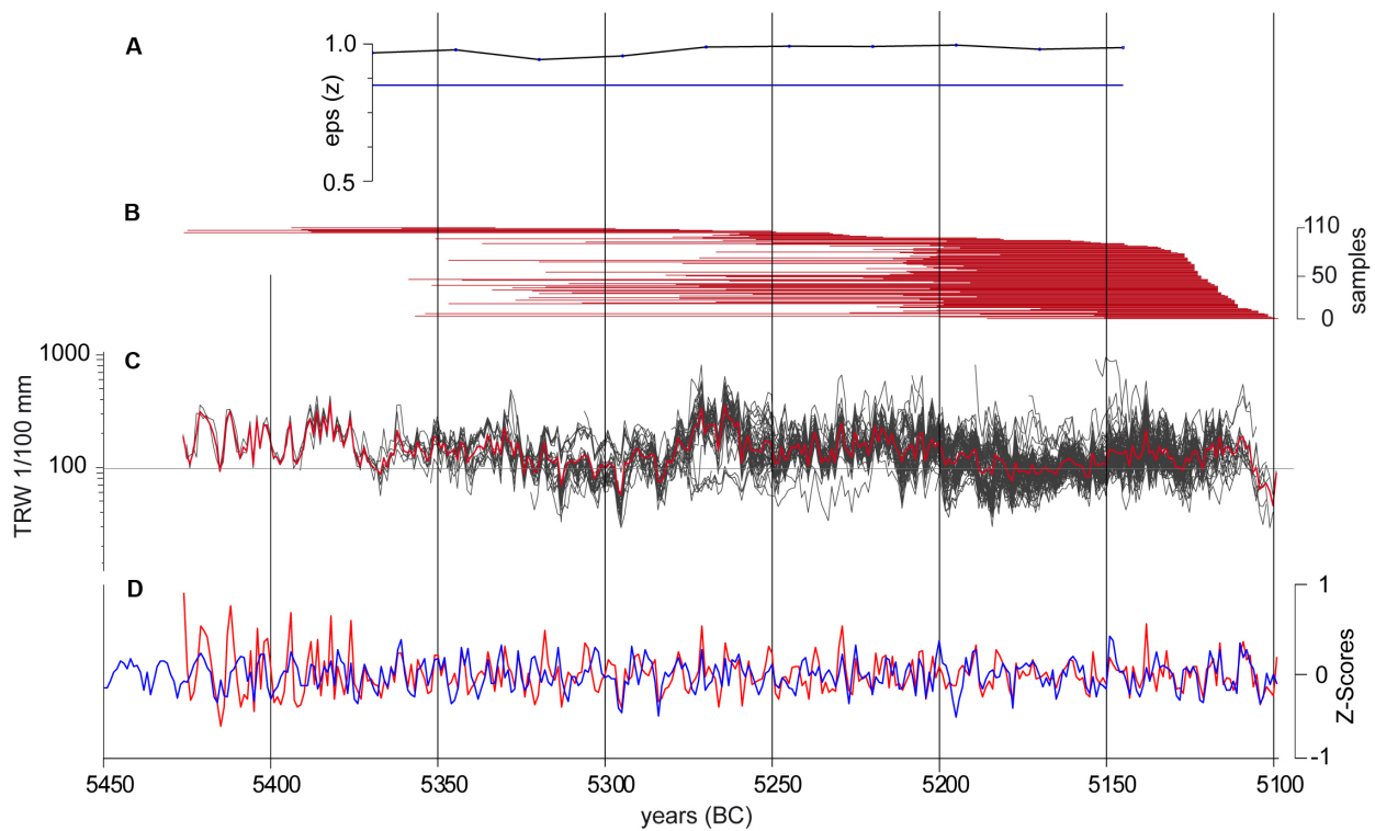
Figure S13. Synchronization of the 124 Altscherbitz tree-ring series. (A) EPS over 50 years, lagged by 25 years, (B) replication, (C) individual tree-ring series (black) in overlap with mean (red), (D) mean chronology in overlap with the chronology from the Main river valley after 10-year smoothing [1].
