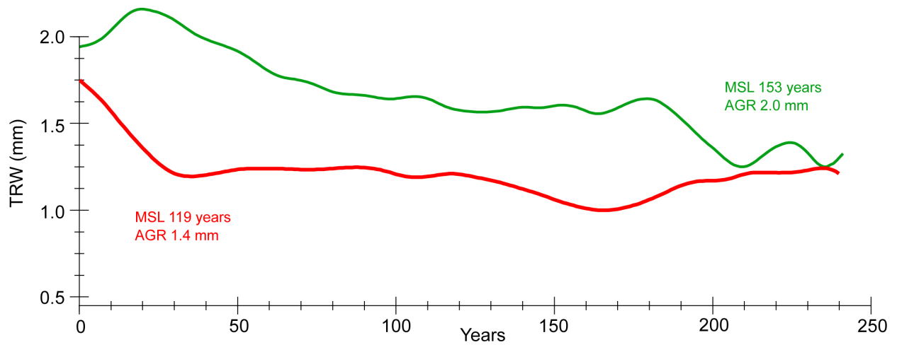
Figure S12. Smoothed regional curves representing the average age trend of recent oaks from Central Eastern Germany (green) and Early Neolithic oaks from the Altscherbitz well construction (red).
