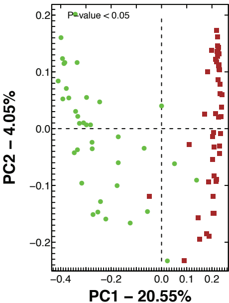
Unweighted Unifrac Bacteria
