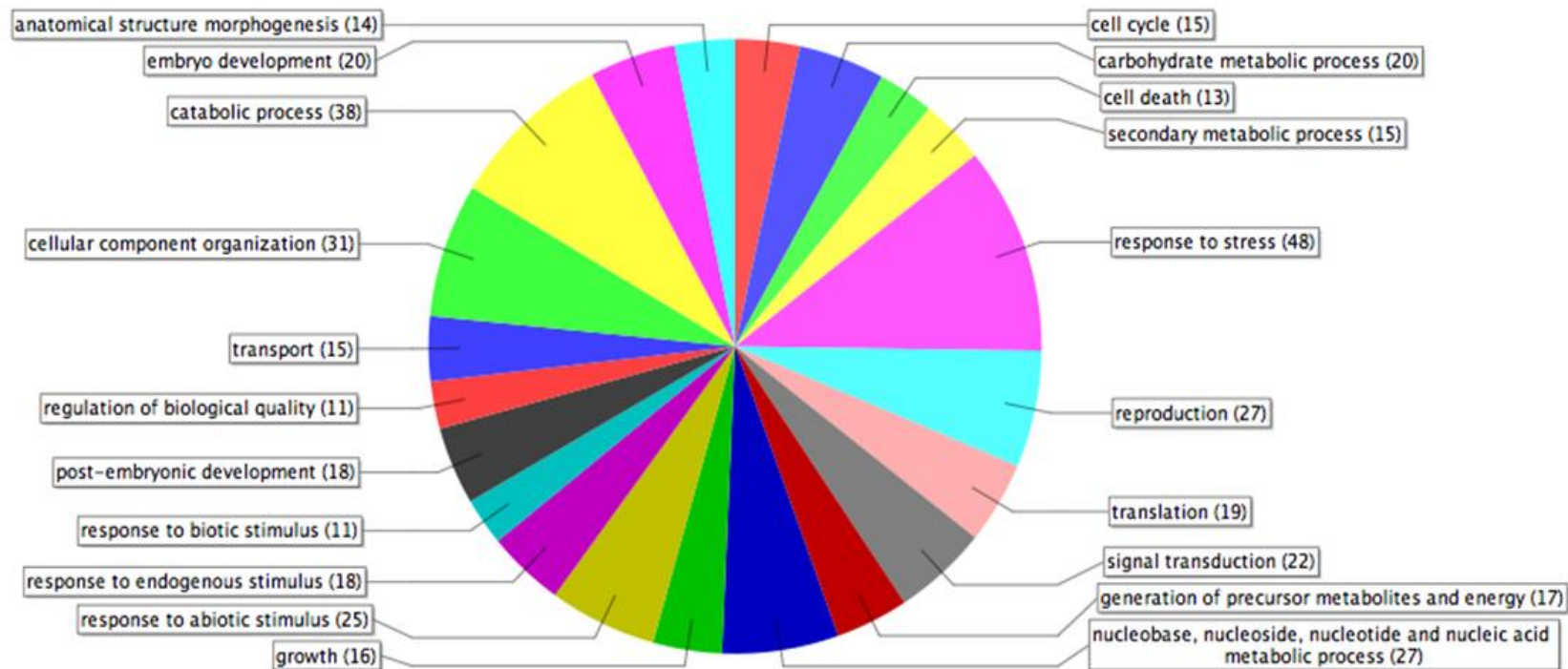
Fig. S3 Resistant related induced (RRI) proteins in wheat NIL with resistant Fhb1 allele following F. graminearum inoculation.
