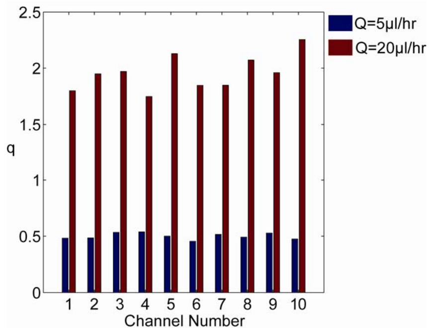
Figure S2. Channel flow rates ( q ) for 2 different input flow rates ( Q ) in an array of ten 50\mu\text{m} wide channels.
