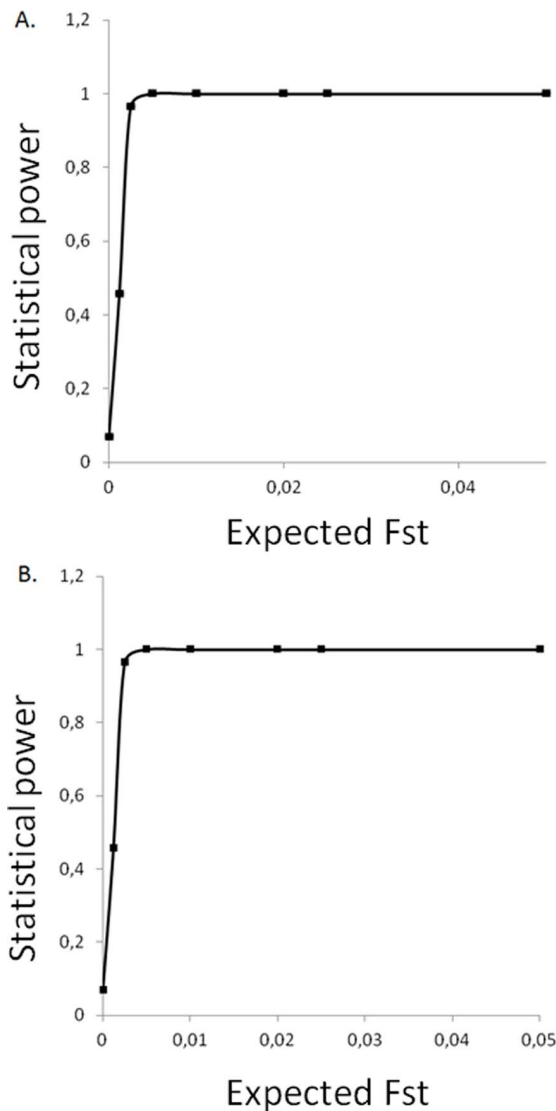
Figure 2. Statistical power in detection of significant genetic differentiation. Statistical power is given as calculated by POWSIM 4.1 (Ryman and Palm 2006). A. Simulated sampling of N_e = 1000 into six populations reflecting sample sizes of A_{VCG} , A_{PVS} , P_{VCG} , P_{PVS} , M_{BOU} , M_{PUY} sampling groups. B. Simulated sampling of N_e = 1000 into three populations reflecting sample sizes of A, P and M overwintering strategies. doi:10.1371/journal.pone.0072997.g002
