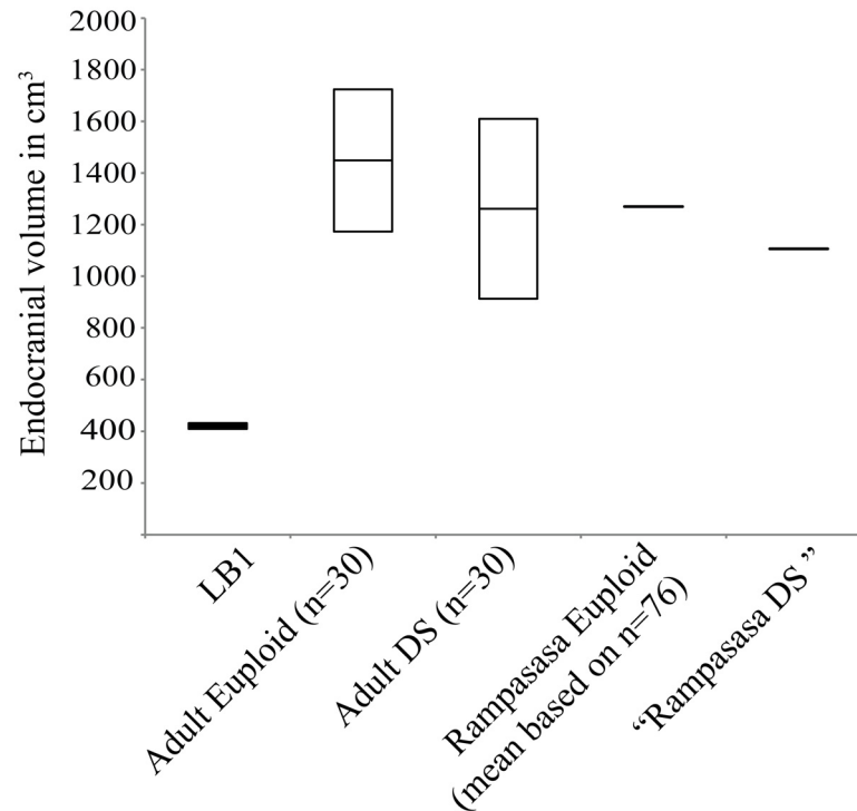
Fig 2. Box plot of endocranial volumes. The DS and matched euploid clinical samples are from Aylward, Habbak [73]. The center line represents the average value while the box captures \pm 2 SDs. The mean value for the Rampasasa population is from Henneberg, Eckhardt [25]. The average value of an individual with DS from the Rampasasa population ("Rampasasa DS") was estimated as 87% of the euploid value, based on the relationship between the matched DS and euploid samples in Aylward, Habbak [73].
