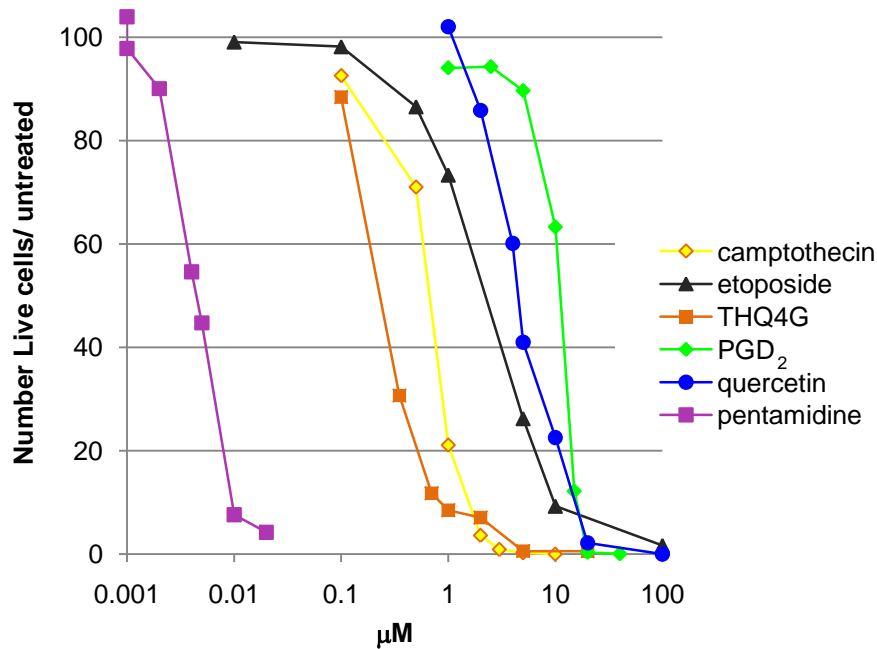
Fig. S1. Titration curves for drugs. Triplicate cultures of BF were analyzed following 24 hour treatments with the indicated concentrations of drugs. The Y axis represents the number of live cells compared to the untreated control. The number of live cells was determined by a combination of Coulter counting and the percent live cells as determined by calcein/ ethidium homodimer staining as revealed by flow cytometry as described in Methods.
