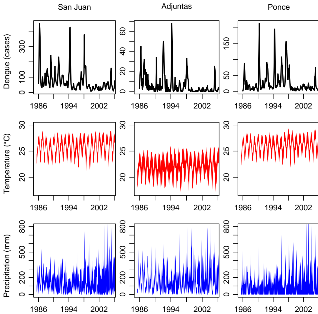
Figure S1. Local time series. Monthly dengue incidence, temperature, and precipitation for 3 municipalities. San Juan is a large urban municipality on the North coast near photo A in Figure 2. Adjuntas is a small rural municipality in the central mountains near photo B in Figure 2. Ponce is a large mostly-urban municipality on the South coast near photo C in Figure 2. Temperature and precipitation represent the range of values produced in the weather models. High variability in predicted precipitation is evident.
