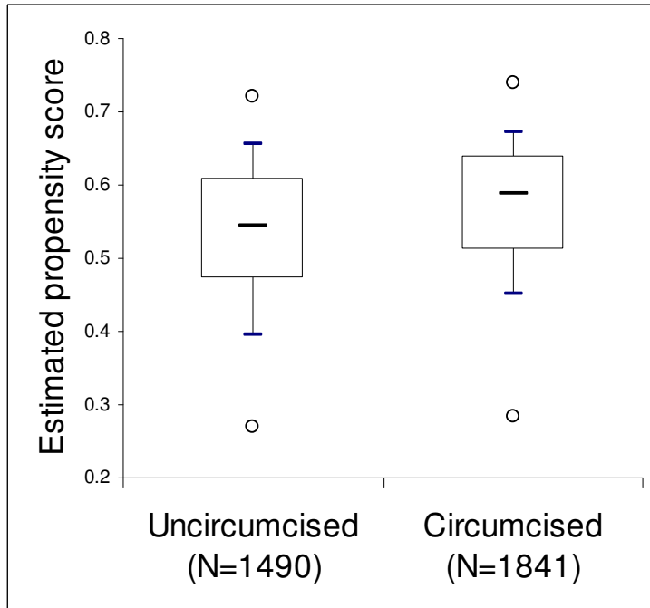
Figure S2: Boxplots of estimated propensity scores by circumcision status: minimum, first decile, lower quartile, median, upper quartile, ninth decile, and maximum
