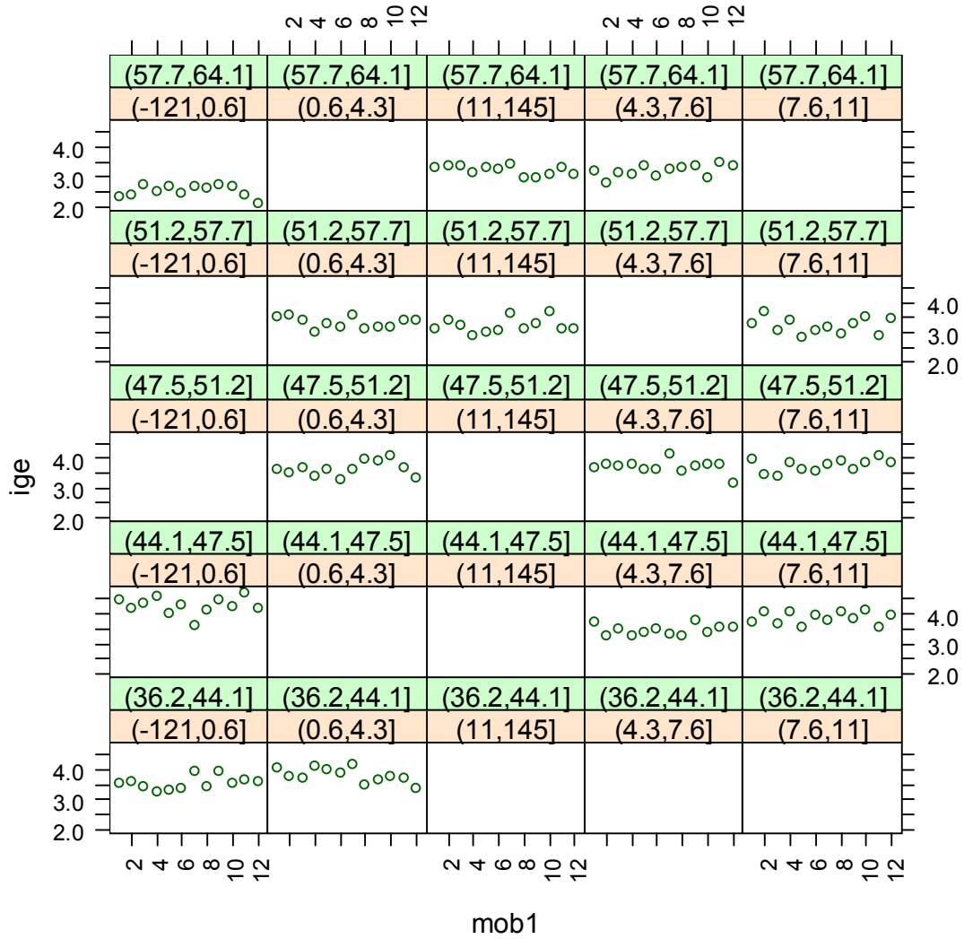
Figure O-17: Median log total IgE by month of birth and latitude/longitude.
