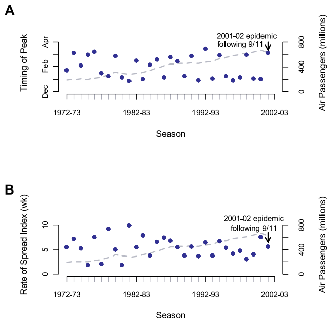
Figure 1. Patterns of Timing (A) and Spread (B) of 30 Influenza Epidemics in the US, Together with Trends in Air Travel Statistics
