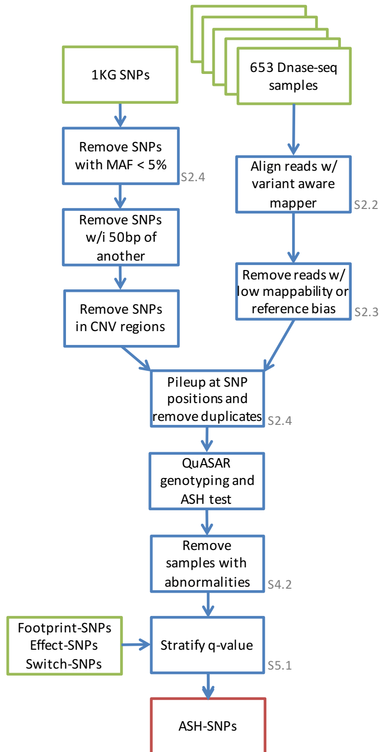
Figure S2: Flowchart detailing ASH analysis pipeline. Numbers next to boxes refer to the corresponding section in the Supplement.
