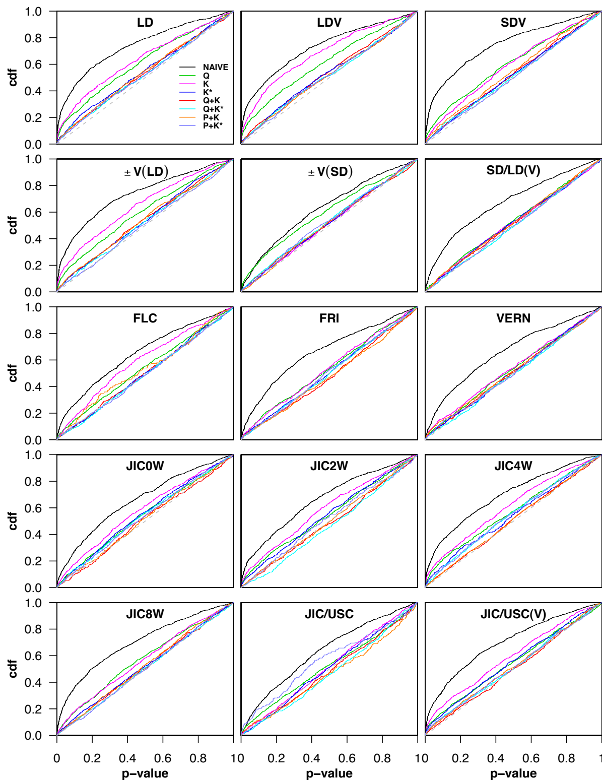
Figure S2: The cumulative distribution of p-values in genome-wide scans for all phenotypes. The different curves correspond to different approaches for correcting for population structure (described in Table 2). Without correction for population structure, all p-value distributions are strongly skewed towards significance. These results are for associations between phenotype and haplotypes (cf. Figure 2).
