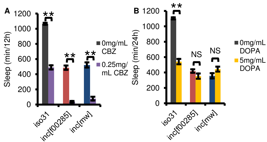
Figure S10: inc functions in a dopaminergic arousal pathway.
