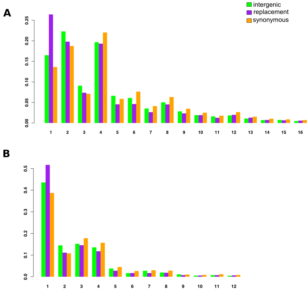
Figure S5: Minor allele frequency spectrum for the S. meliloti chromosome. The MAF spectrum for the full set of strains (A) shows a mode at 4. Reducing the sample to just the 24 strain lineage brings the MAF spectrum closer to neutral expectations (B).
