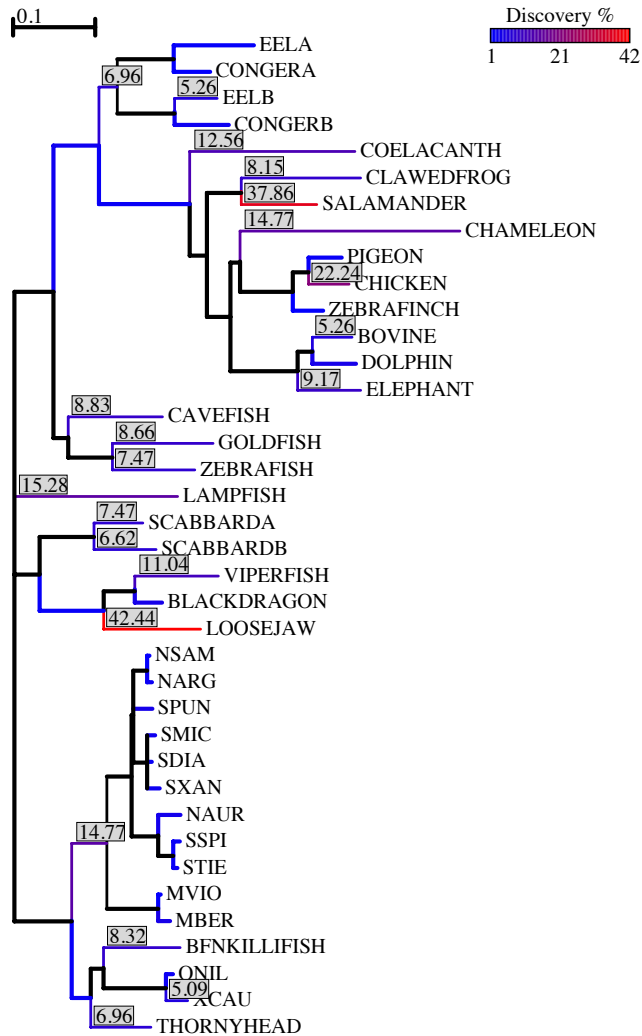
30% of sites. Weakly negatively selected background ( \omega = 0.5 )
