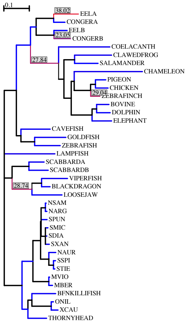
50% of sites. Strongly negatively selected background ( \omega = 0.1 )
