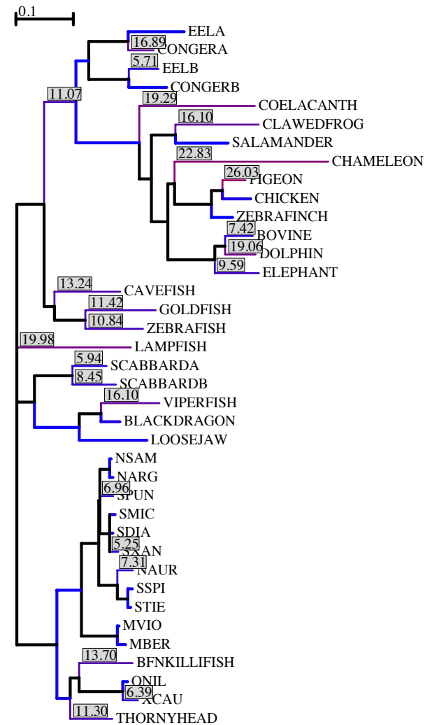
20% of sites. Neutral background ( \omega = 1 )
