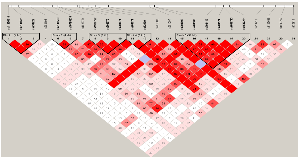
Caribbean Hispanics
