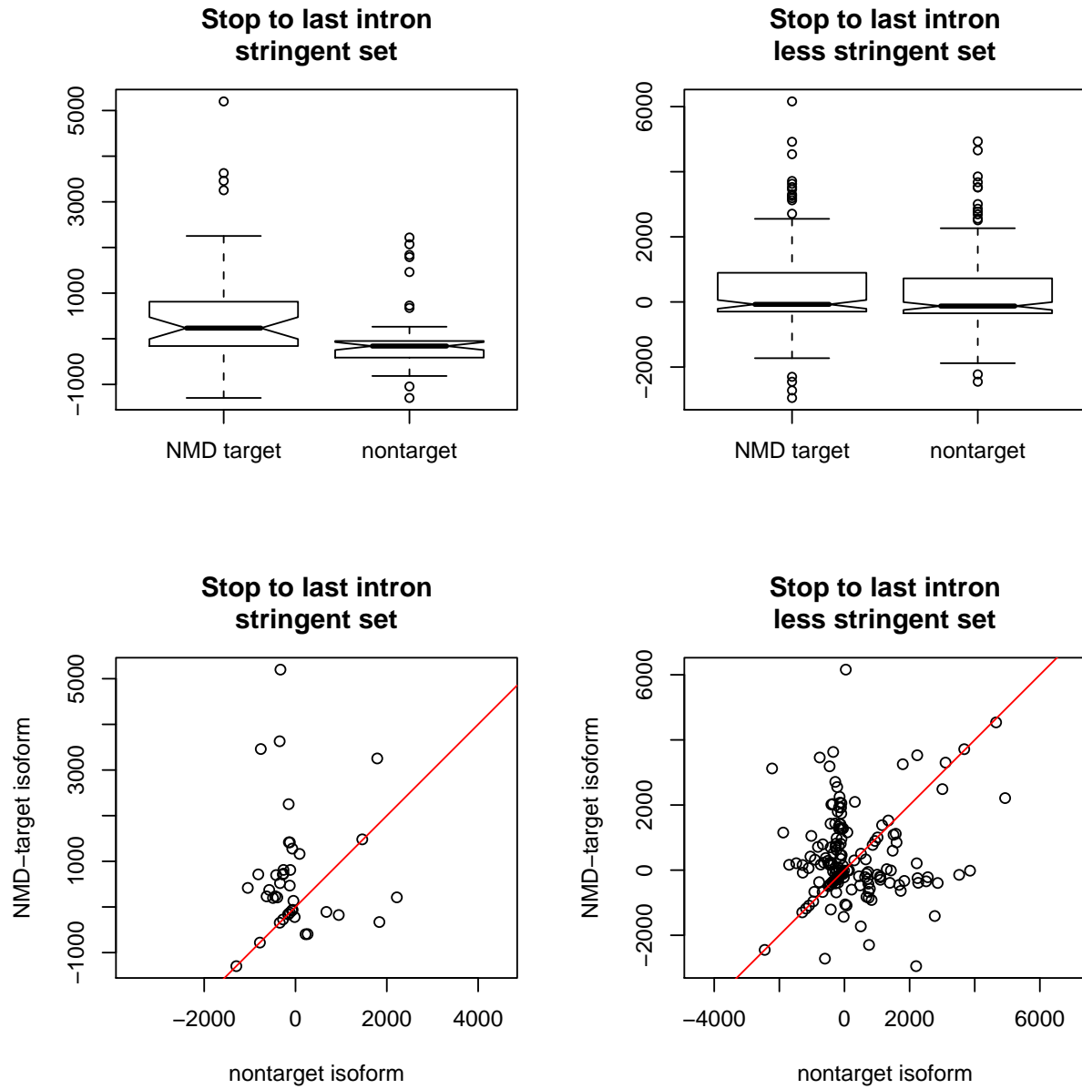
Figure S21. Distance from stop codon to final intron. As Figure S9 for the feature “distance from stop codon to final intron.” CG11100 did not have any introns and is not assigned a value.
