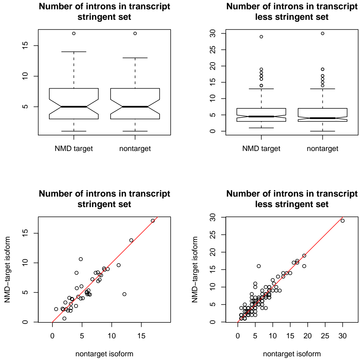
Figure S18. Number of introns in transcript. As Figure S9 for the feature “number of introns in transcript.” The bottom left scatterplot has been jittered.
